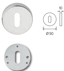
Bocchetta foro chiave. Sottorosetta in plastica. Escutcheon with key hole. PVC under-construction.
