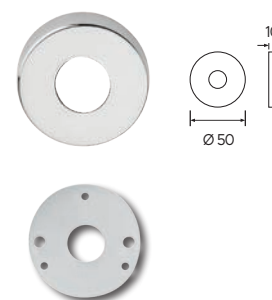
Bocchetta foro wc. Sottorosetta in plastica. Escutcheon with wc hole. PVC under-construction.
