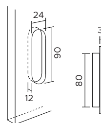
fresatura per nicchia milling for flush handle
