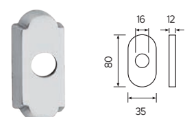
Rosetta DKA. DKA cover.
