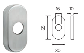
Rosetta DK. DK cover.
